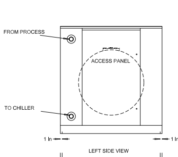
LEFT SIDE VIEW Qty (8) 1/2" Mounting Holes
