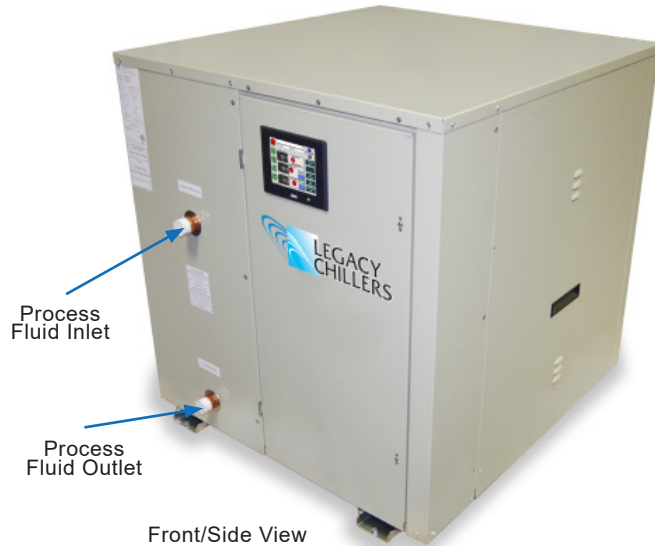
Front/Side View
