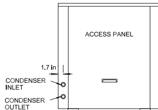
BACK VIEW
