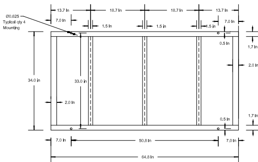
FRAME LAYOUT
