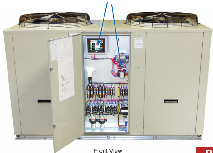
Front View (Electrical Cabinet Open)
