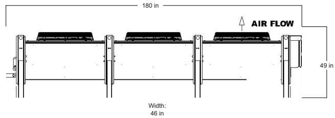
OC Refrigerant Connections: Discharge Line- 1 1/8" (2), Liquid Line- 5/8" (2)
