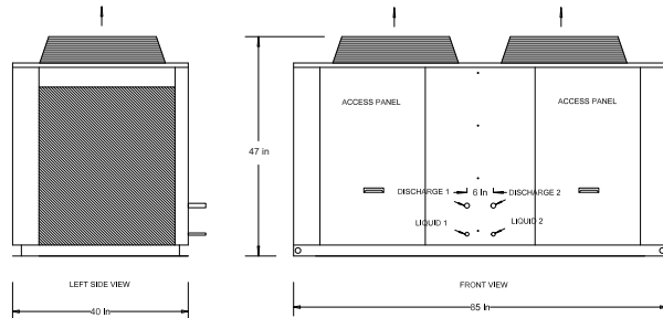
OC Refrigerant Connections: Discharge Line- 7/8" (2), Liquid Line- 5/8" (2)
