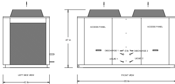
OC Refrigerant Connections: Discharge Line- 7/8" (2), Liquid Line- 1/2" (2)
