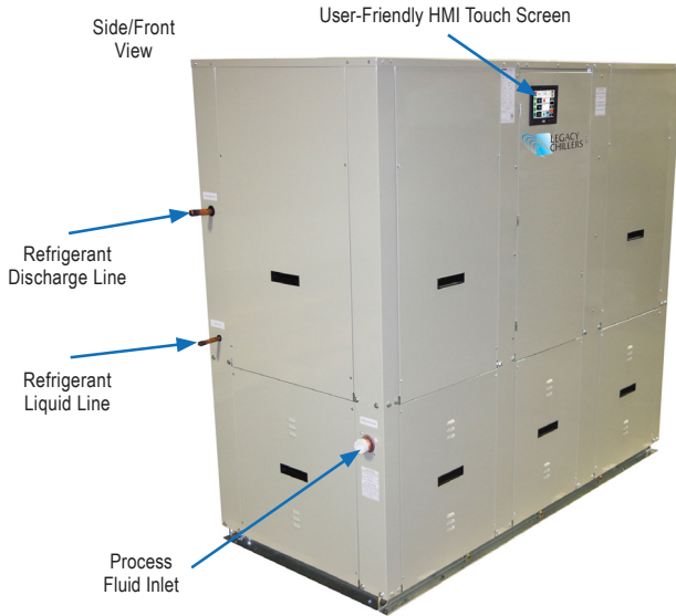
OC Refrigerant Connections: Discharge Line- 1 1/8", Liquid Line- 5/8"
