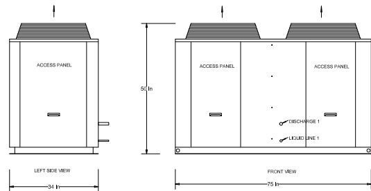
OC Refrigerant Connections: Discharge Line- 1 1/8", Liquid Line- 5/8"
