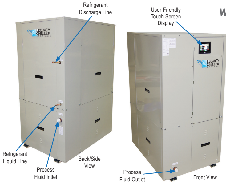
OC Refrigerant Connections: Discharge Line- 1/2", Liquid Line- 3/8"
