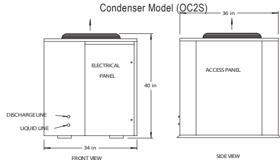
OC Refrigerant Connections: Discharge Line- 1/2", Liquid Line- 3/8"
