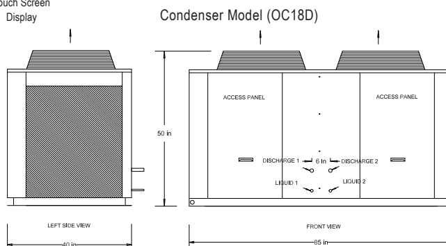
OC Refrigerant Connections: Discharge Line- 7/8" (2), Liquid Line- 5/8" (2)
