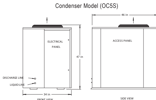
OC Refrigerant Connections: Discharge Line- 3/4", Liquid Line- 1/2"
