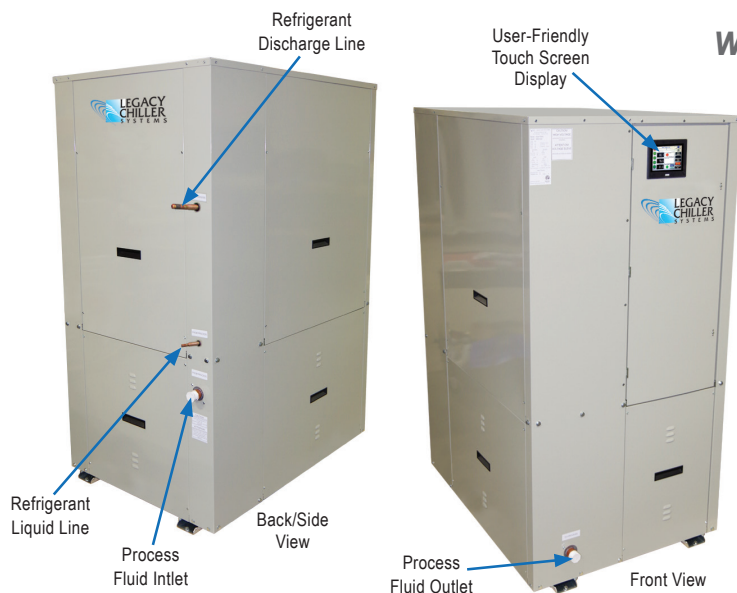
OC Refrigerant Connections: Discharge Line- 3/4", Liquid Line- 1/2"
