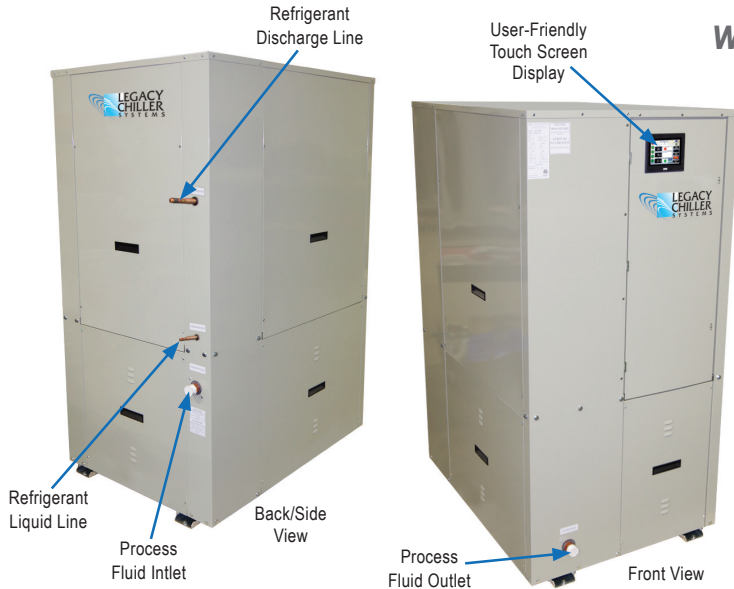
OC Refrigerant Connections: Discharge Line- 1/2", Liquid Line- 3/8"
