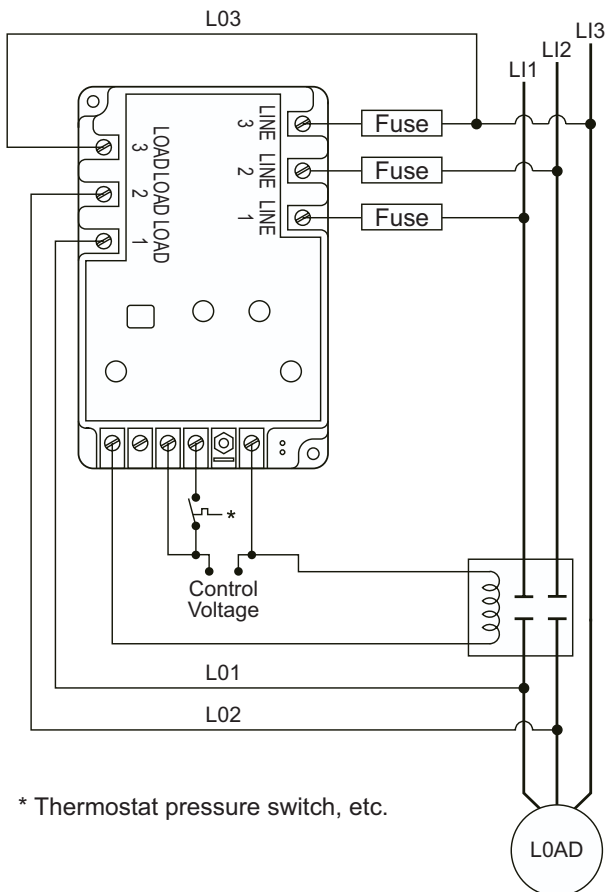
2-Pole Contactor
