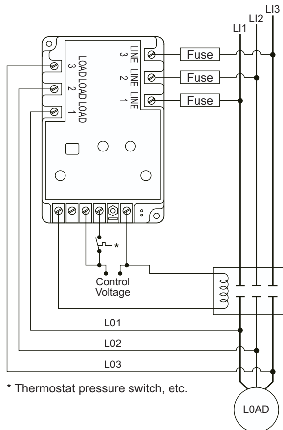
3-Pole Contactor
