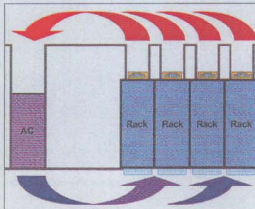
Figure 5: High-density heat containment system.
